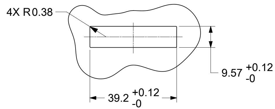
RECOMMENDED MOUNTING PATTERN
