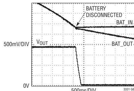
Battery Connect Transient
