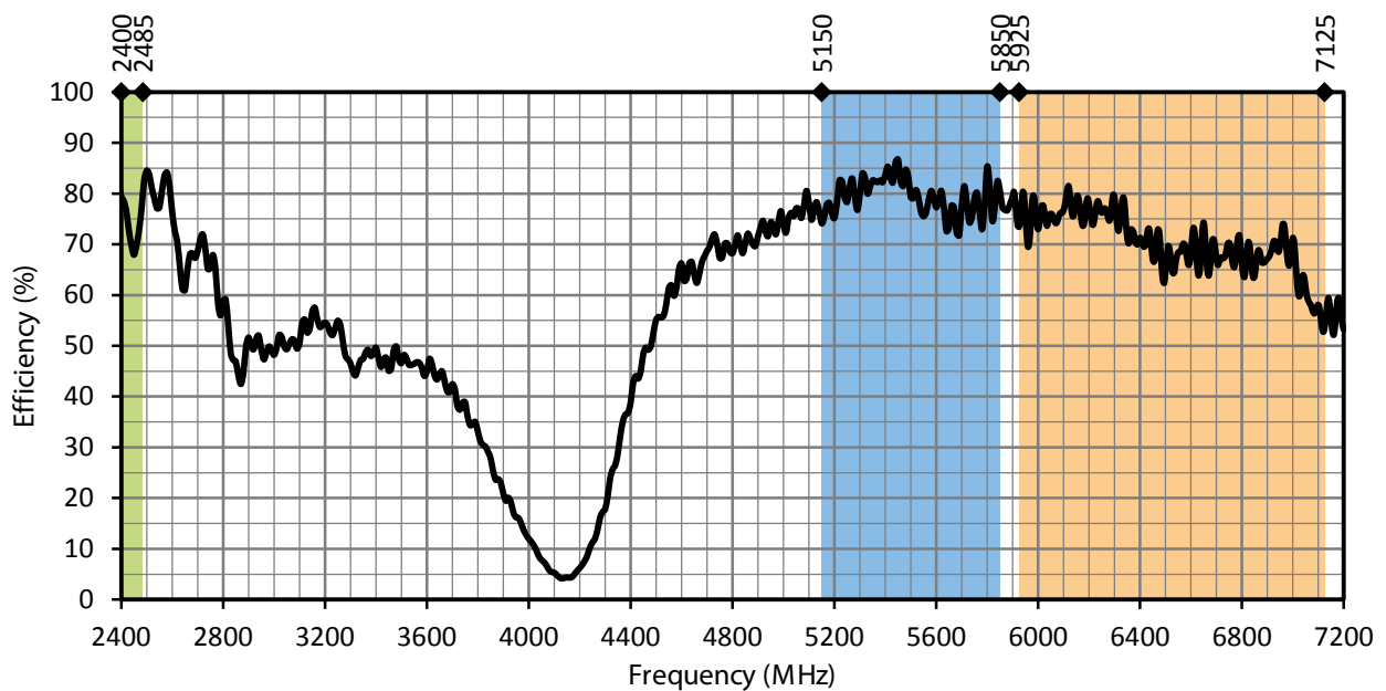
Figure 8. ANT-W63WS4-ccc Antenna Efficiency, Straight
