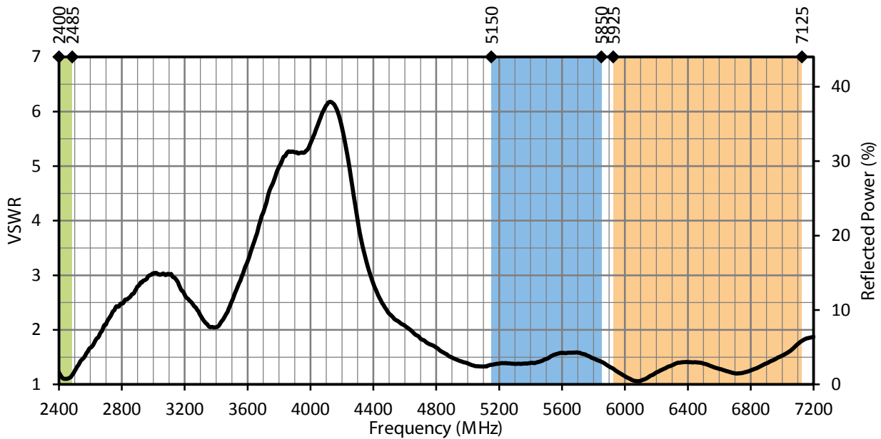
Figure 4: ANT-W63WS4-ccc VSWR, StraightHighlights
