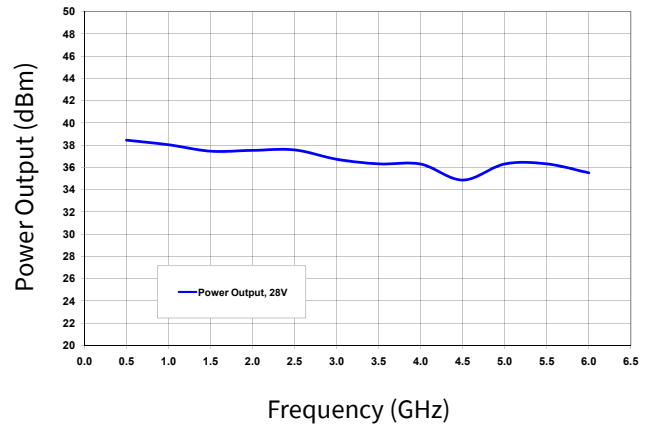
Figure 2. Power Output vs Frequency V_{DD} = 28\text{ V} , P_{IN} = 23\text{ dBm}
