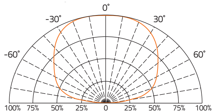
Fig. 6 Direct Radiation
