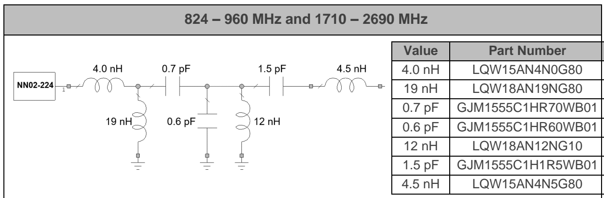
Figure 2 – Matching Network implemented in the evaluation board (Error! Reference source not found.).
