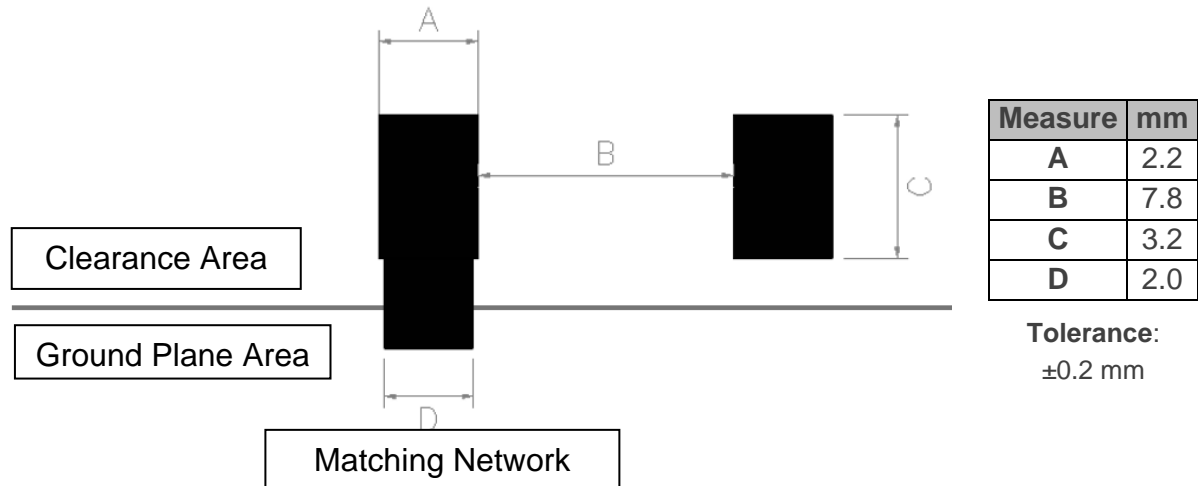
Figure 17 – Footprint dimensions for the single booster.
