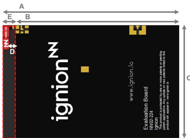
Figure 13 – EB_NN02-224-CR80-2400 in CR80 standard format. Evaluation Board providing operation from 2.4 GHz to 2.5 GHz.
