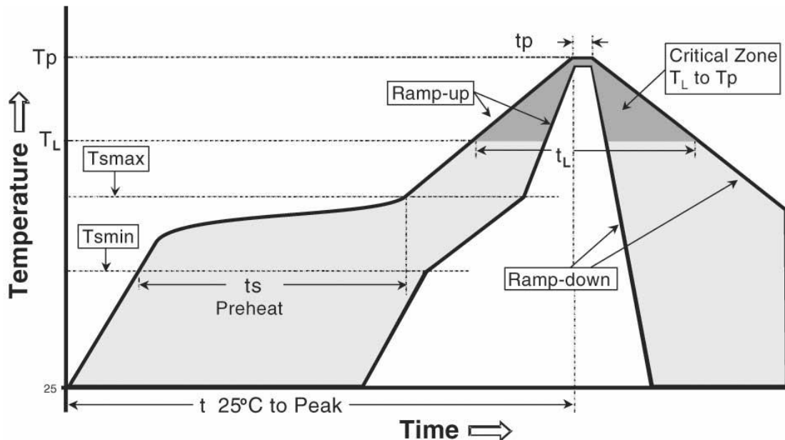
Figure 20 – Temperature profile.
