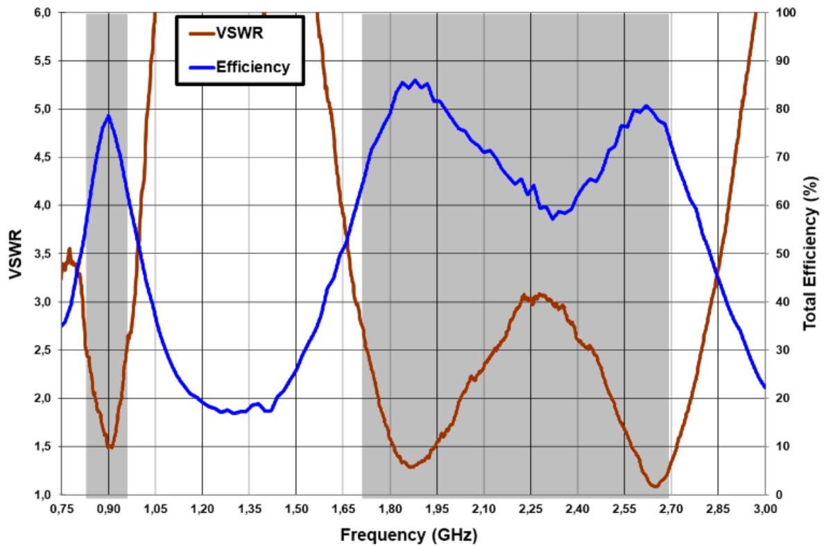
Figure 3 – VSWR and Total Efficiency for the 824 – 960 MHz frequency range and for the 1710 – 2690 MHz frequency range (from the evaluation board ( Error! Reference source not found. )).
