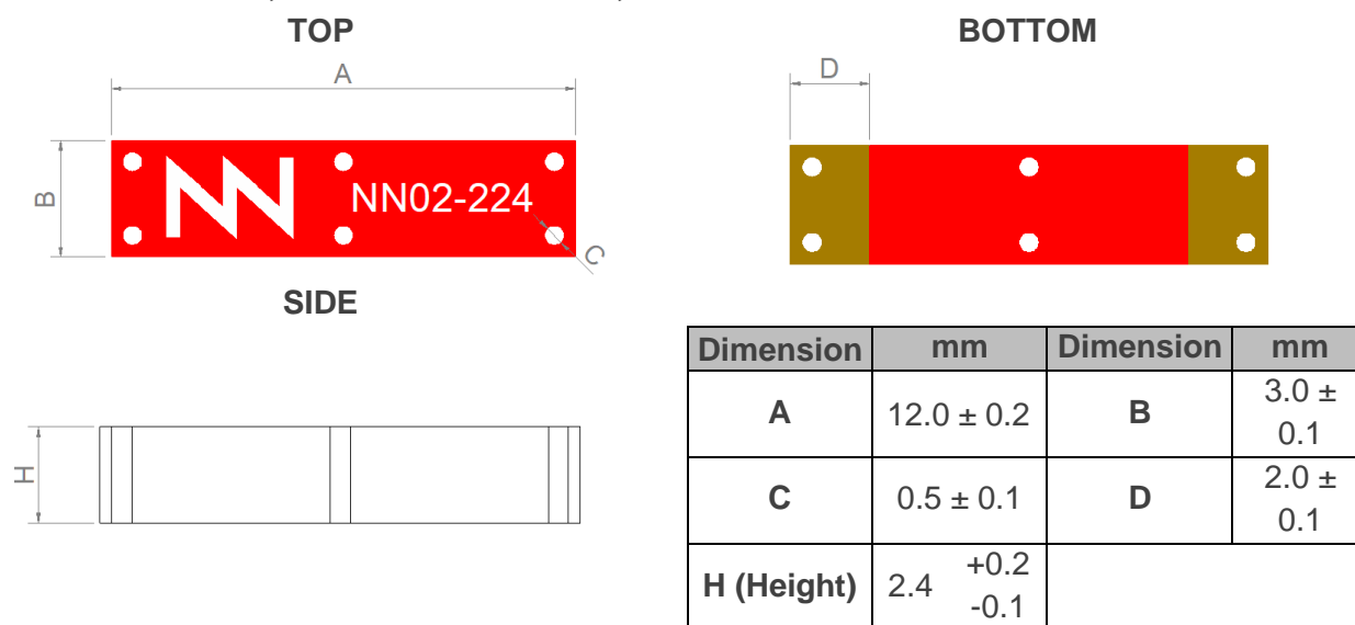
Figure 16– RUN mXTEND ™ antenna booster dimensions and tolerances.
