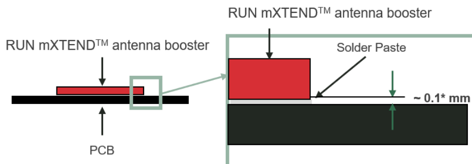
Figure 19 – Soldering Details.
