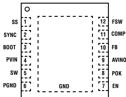
ER3110DI (12 LD 4X3 DFN) TOP VIEW
