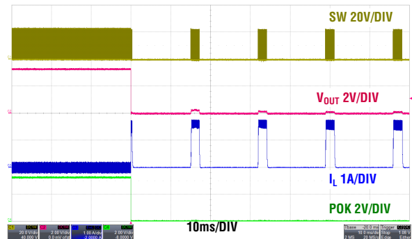
FIGURE 38. OVERCURRENT PROTECTION HICUP, PWM
