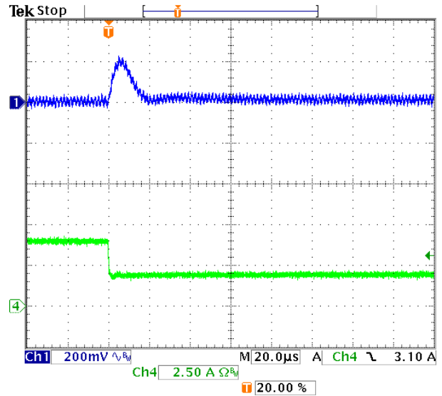
Fig. 12: Output voltage response for V_{out}=8V to negative load current step change from 4A to 2A with slew rate of -5A/\mu s at V_{in}=24V . C_o=22\mu F \times 2 ceramic + 1\mu F ceramic.
