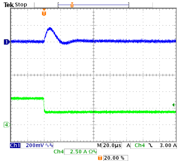
Fig. 16: Output voltage response for V_{out}=3.3V to negative load current step change from 4A to 2A with slew rate of -5A/\mu s at V_{in}=24V . C_o=47\mu F \times 2 ceramic + 1\mu F ceramic.
