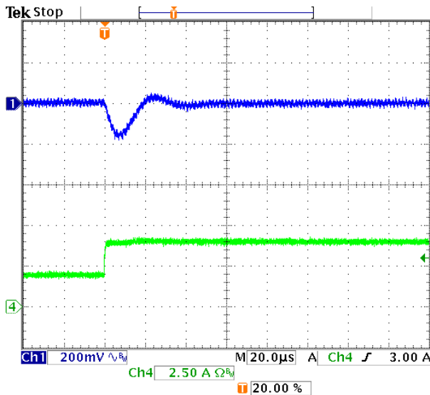
Fig. 15: Output voltage response for V_{out}=3.3V to positive load current step change from 2A to 4A with slew rate of 5A/\mu s at V_{in}=24V . C_o=22\mu F \times 2 ceramic + 1\mu F ceramic.
