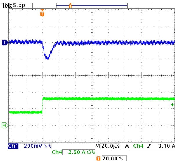
Fig. 11: Output voltage response for V_{out}=8V to positive load current step change from 2A to 4A with slew rate of 5A/\mu s at V_{in}=24V . C_o=22\mu F \times 2 ceramic + 1\mu F ceramic.
