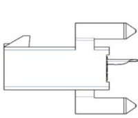
Example header with "formed" terminals
