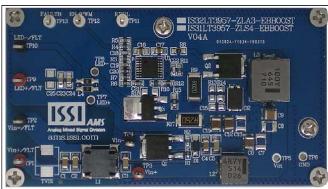
Figure 1 Photo of IS32LT3957/IS31LT3957 Boost Evaluation Board
