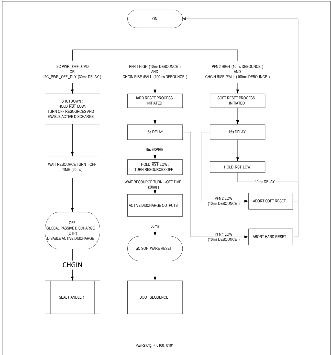
Figure 1c. PwrRstCfg = 0100 or 0101
