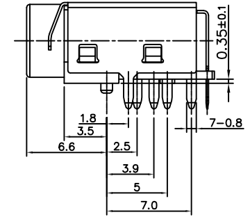
MATE PLUG
