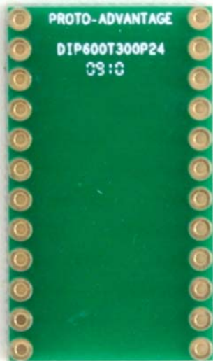
2D Top View (Pins Unassembled)
