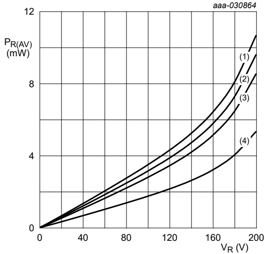
T_j = 175^\circ\text{C} (1) \delta = 1 ; DC (2) \delta = 0.9 (3) \delta = 0.8 (4) \delta = 0.5
