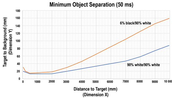
Figure 25. Minimum Object Separation for 50 ms Response Time
