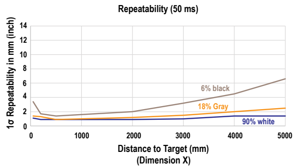
Figure 24. Repeatability for 50 ms Response Time
