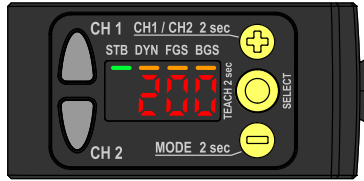
Figure 3. Button Layout
