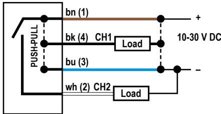
Figure 12. Channel 2 as PNP Discrete or PFM Output
