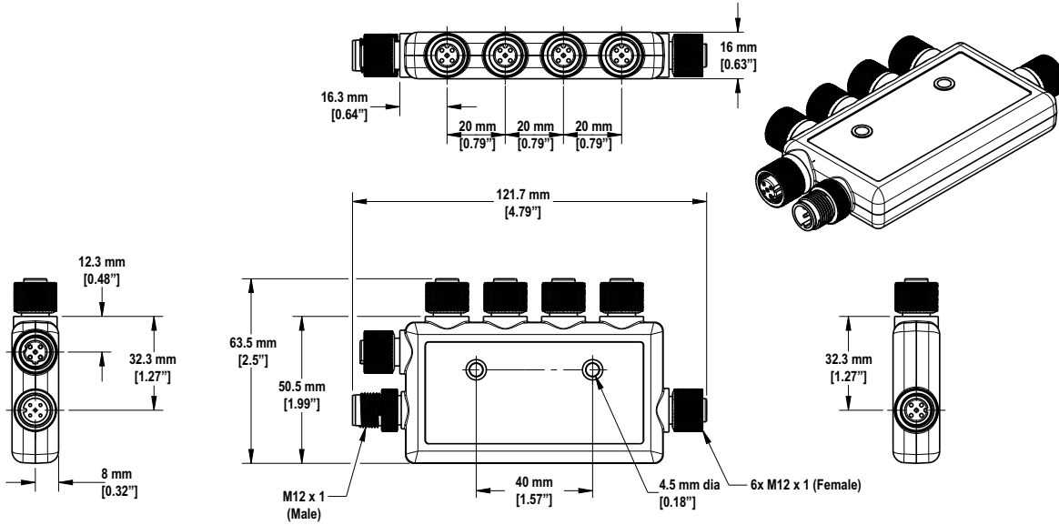
Figure 2: DXMR90-X1 dimensions
