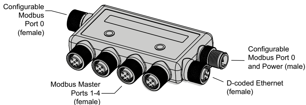
Figure 1: Overview of the DXMR90-X1 Series Controller
