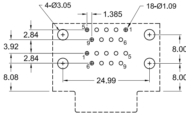
Recommended PC Board Layout (Top Front View)
