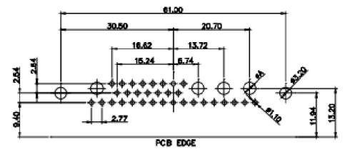
36W4 Female
