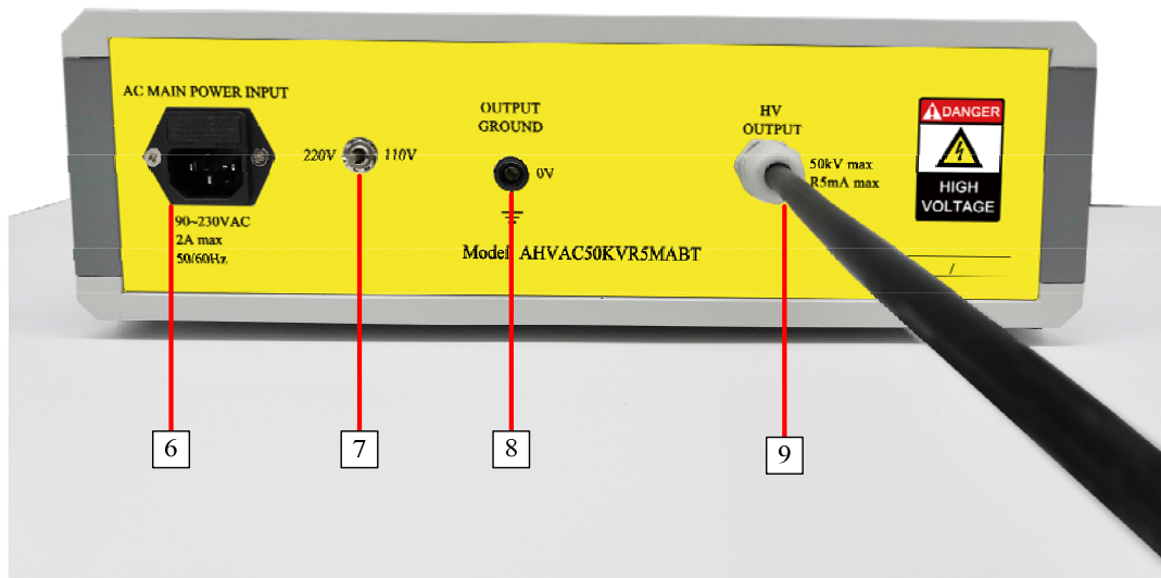
Figure 3. Front Panel
