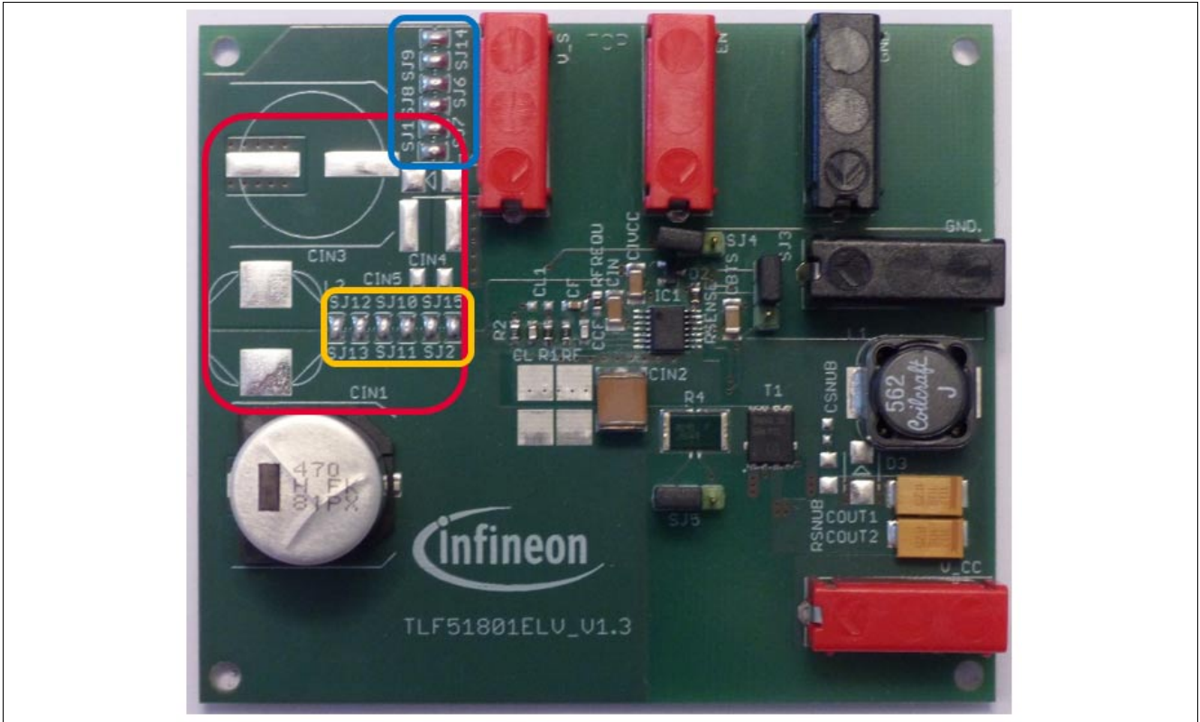
Figure 9 Input filter
