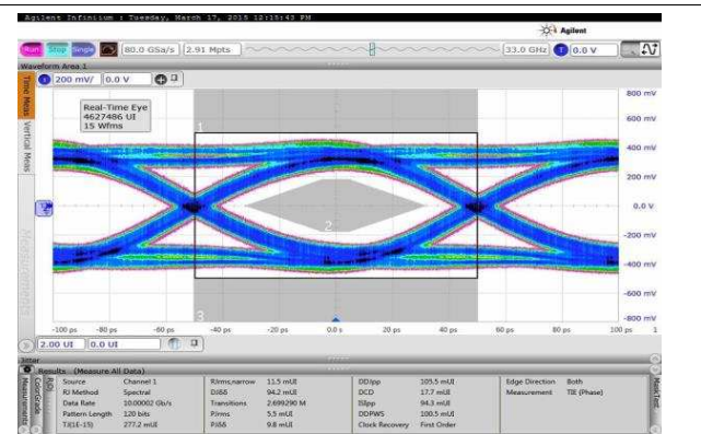
Figure 81. Eye Diagram at 10-Gbps Bit Rate with Increased Output Swing
