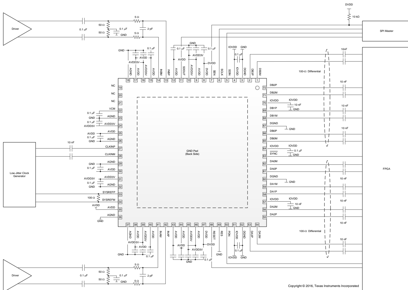
Figure 132. AC-Coupled Receiver
