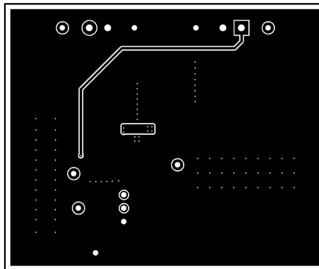
Figure 5-3. Bottom Layer
