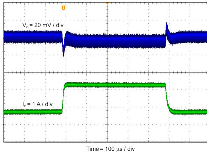
Figure 4-5. Load Transient Response, 25% to 75% Load Step
