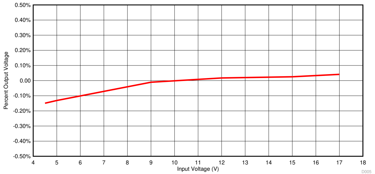
Figure 4-4. Line Regulation
