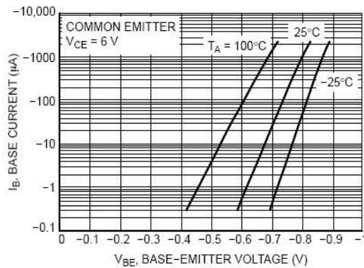
Fig. 5. Base-Emitter Voltage
