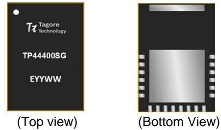
Figure 1 Device Image (22pin 5x7x0.85 mm QFN Package)
