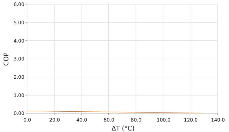
Coefficient of Performance (COP = Qc/Pin) Thot = 27 °C | Current = 1.4 Amps
