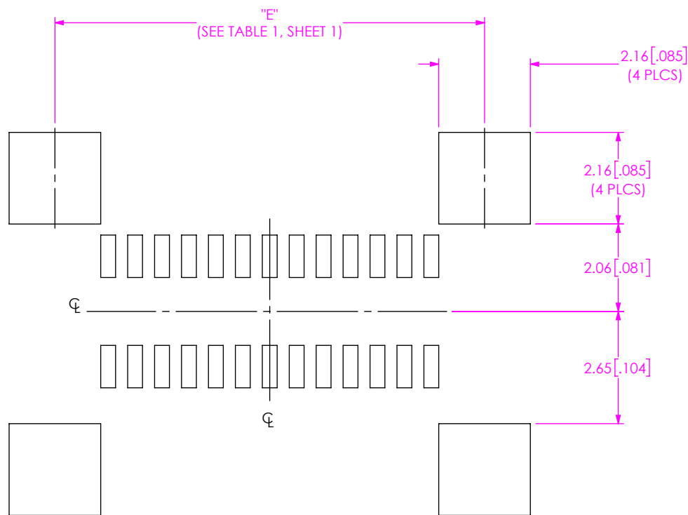
FIG 2 ARF6-08-X-D-A-K-TR SHOWN (DIFFERENT AS SHOWN, OTHERWISE SAME AS FIG 1) ALL DIMENSIONS ARE SYMMETRIC ABOUT THE CENTERLINE.
