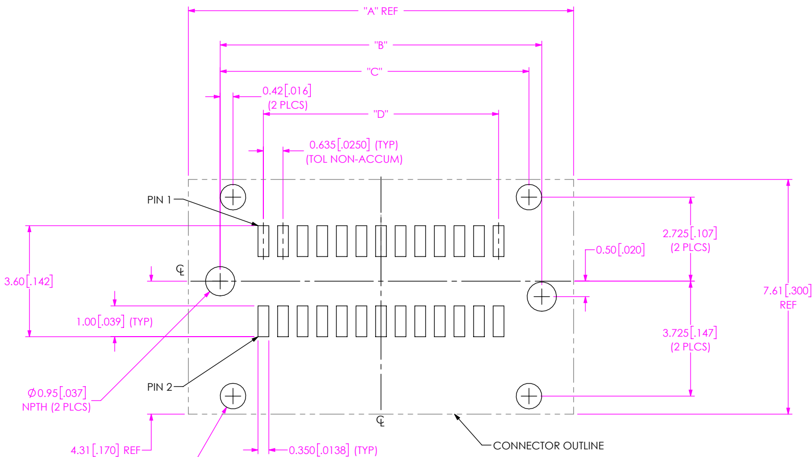
FIG 1 ARF6-08-X-D-A-K-TR SHOWN ALL DIMENSIONS ARE SYMMETRIC ABOUT THE CENTERLINE.
