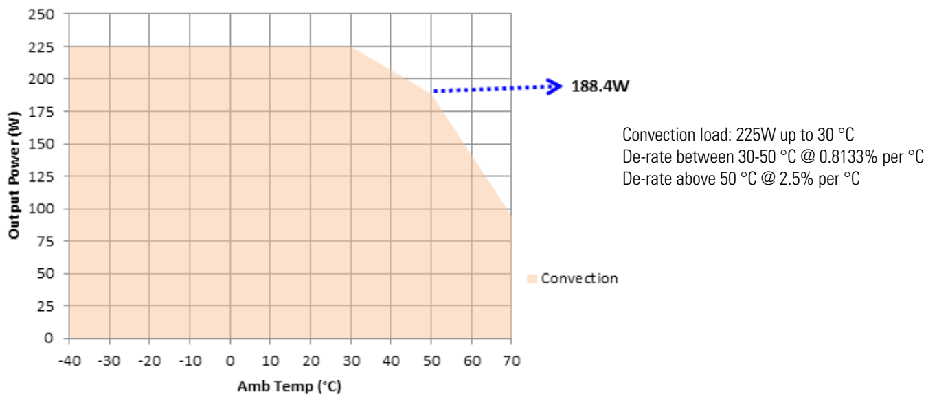
Derating Curve 15 V plain over
