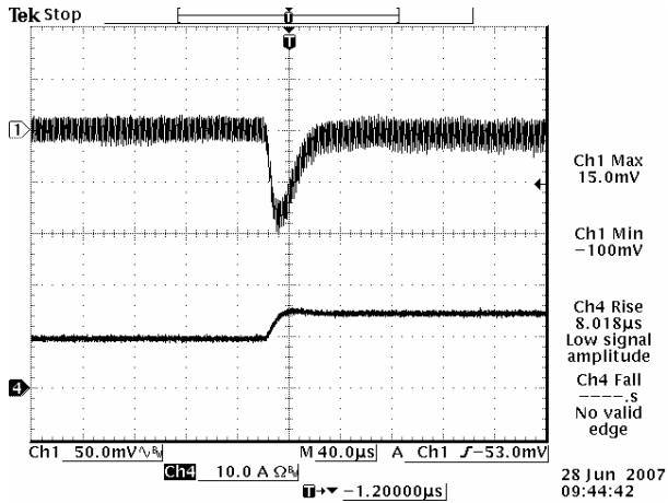
Figure 13. Vout = 5 V, 50%-75% Load Transients
