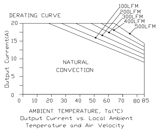
Figure 10. V_{out} = 5 V
