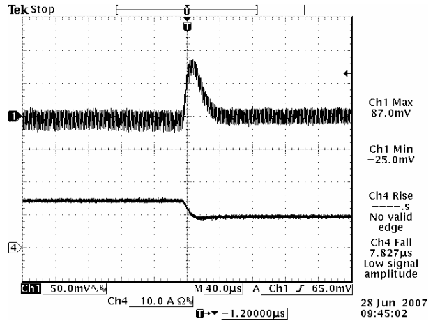
Figure 14. Vout = 5 V, 75%-50% Load Transients
