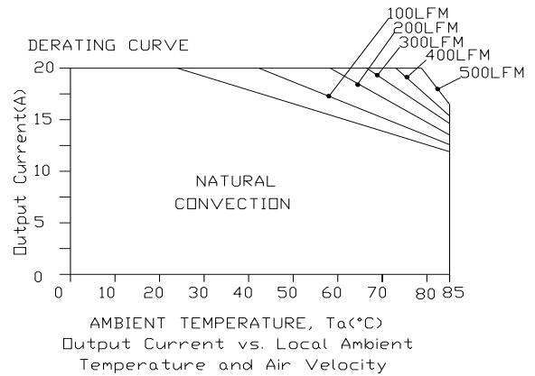
Figure 8. V_{out} = 2.5 V
