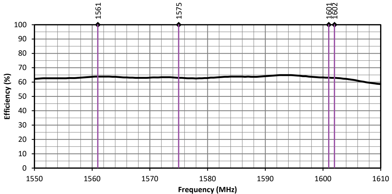
Figure 5. ANT-GNL1-nSP Radiation Efficiency with Frequency Band Highlights
