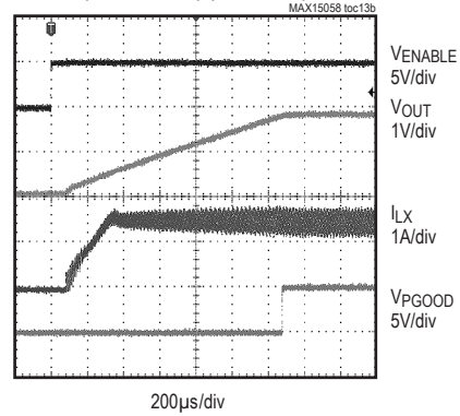
SOFT-START WAVEFORMS (SKIP MODE) ( I_{OUT} = 3A )
