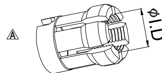
CABLE COLLET
