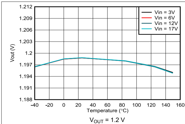
Figure 7-7. Output Voltage Accuracy – VSET Selected
