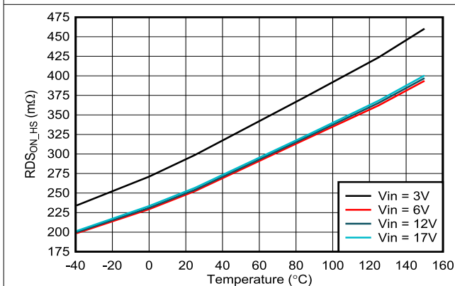
Figure 7-11. High-Side RDS ON vs Temperature
