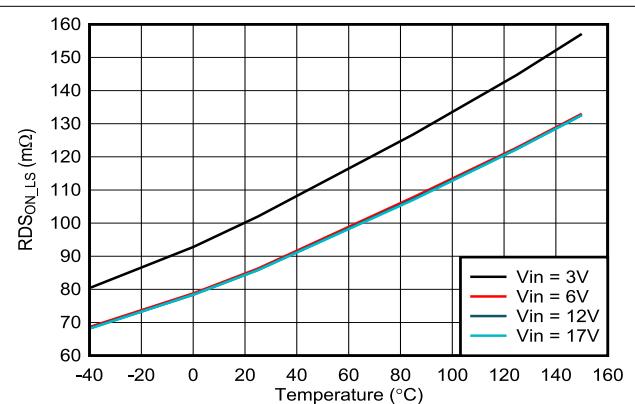
Figure 7-12. Low-Side RDS ON vs Temperature
