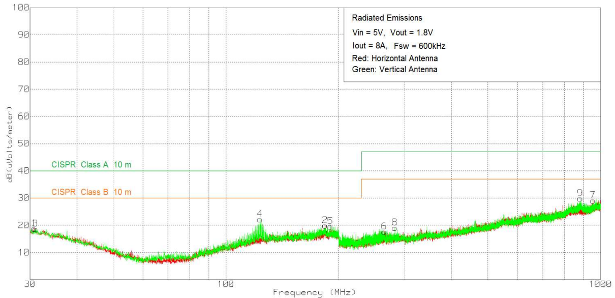
Figure 33. Radiated Emissions 5-V Input, 1.8-V Output, 8-A Load (EN55011 Class B)
