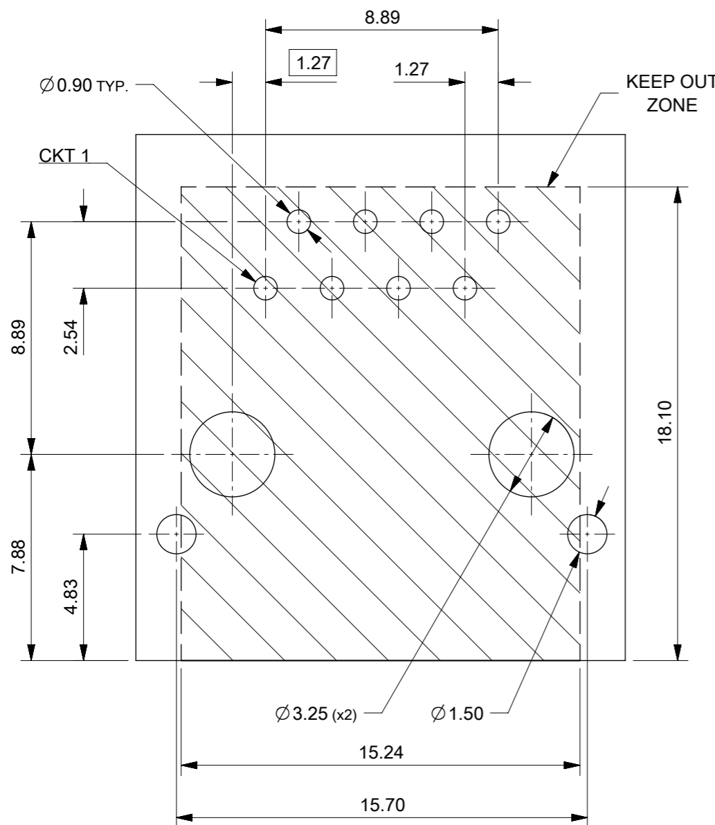
RECOMMENDED P.C. BOARD LAYOUT VIEW FROM COMPONENT SIDE ALL DIMENSIONS REF DIMENSIONS
