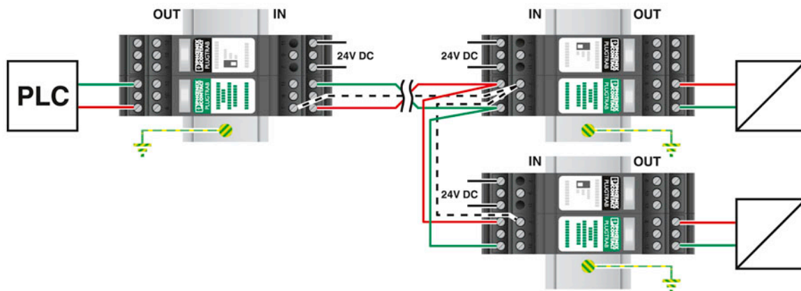
Application drawing
