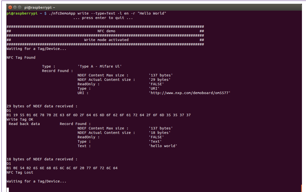
Fig 7. Linux demo application tag writing mode
