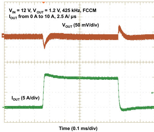
Figure 19. FFCM Load Transients
