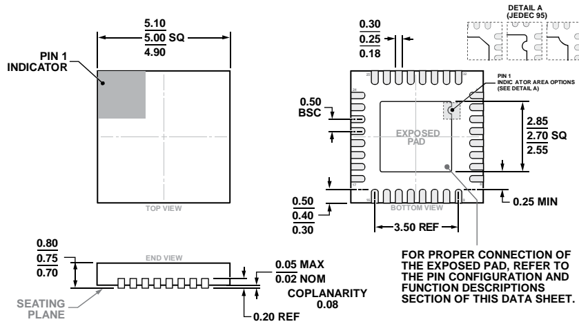
Figure 27. 32-Lead Lead Frame Chip Scale Package [LFCS] 5 mm × 5 mm Body and 0.75 mm Package Height (CP-32-21)
