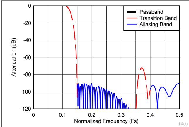
Figure 8-11. Decimate-by-4 Composite Response h4co
