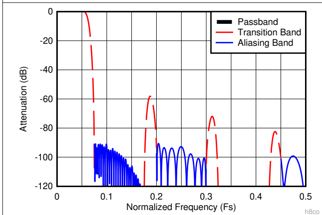
Figure 8-13. Decimate-by-8 Composite Response h8co
