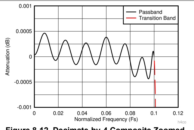
Figure 8-12. Decimate-by-4 Composite Zoomed Pass-Band Response h4co
