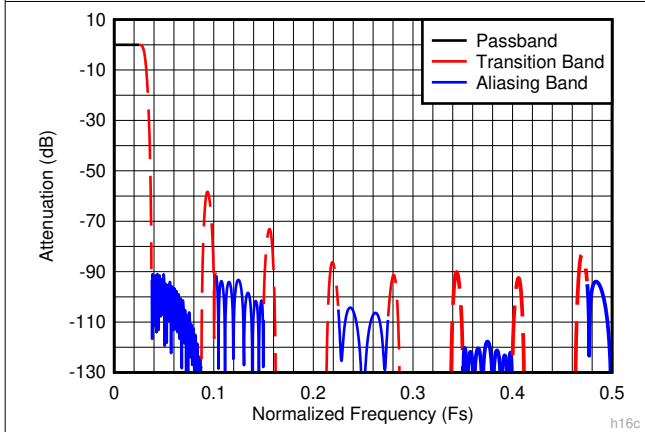
Figure 8-15. Decimate-by-16 Composite Response h16c
