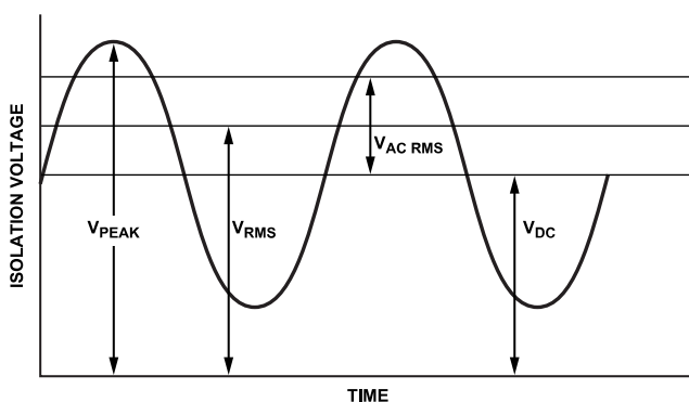
Figure 35. Critical Voltage Example
