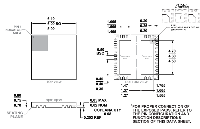
Figure 37. 32-Lead Lead Frame Chip Scale Package [LFCSFP] 6 mm x 6 mm Body and 0.75 mm Package Height (CP-32-32) Dimensions shown in millimeters
