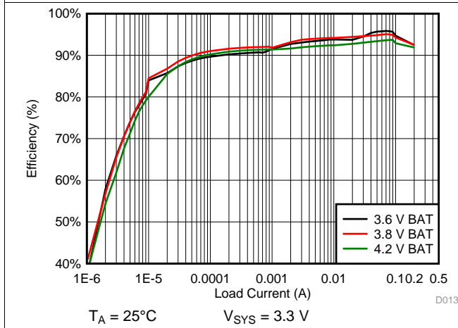
Figure 48. 3.3 V sys System Efficiency
