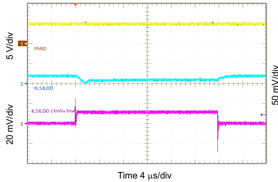
Figure 85. 3.3 V_{LSLDO} Load Transient, 0 to 10 mA
