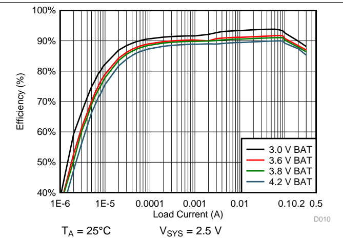
Figure 47. 2.5 V sys System Efficiency
