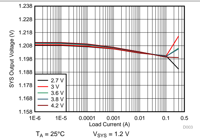
Figure 49. 1.2 V sys Load Regulation
