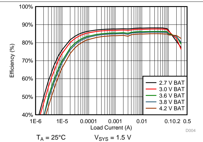
Figure 45. 1.5 V sys System Efficiency
