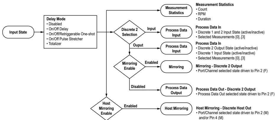
Figure 1: Logic Flow
