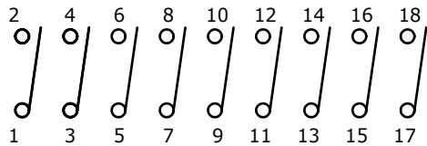
▲ CIRCUIT - 9 POSITION
