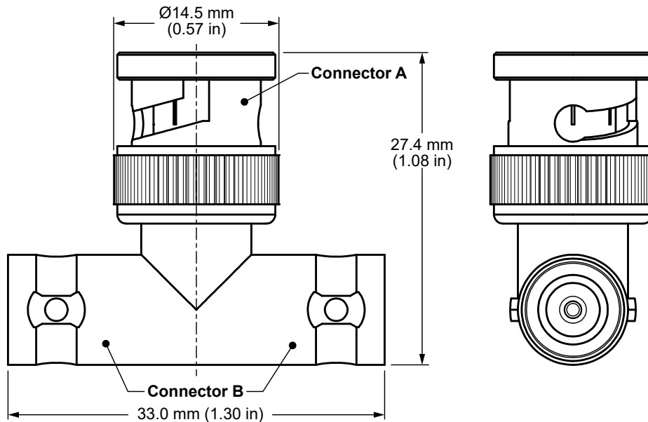
Figure 1. Product Dimensions for the ADP-BNCF-T Adapter
