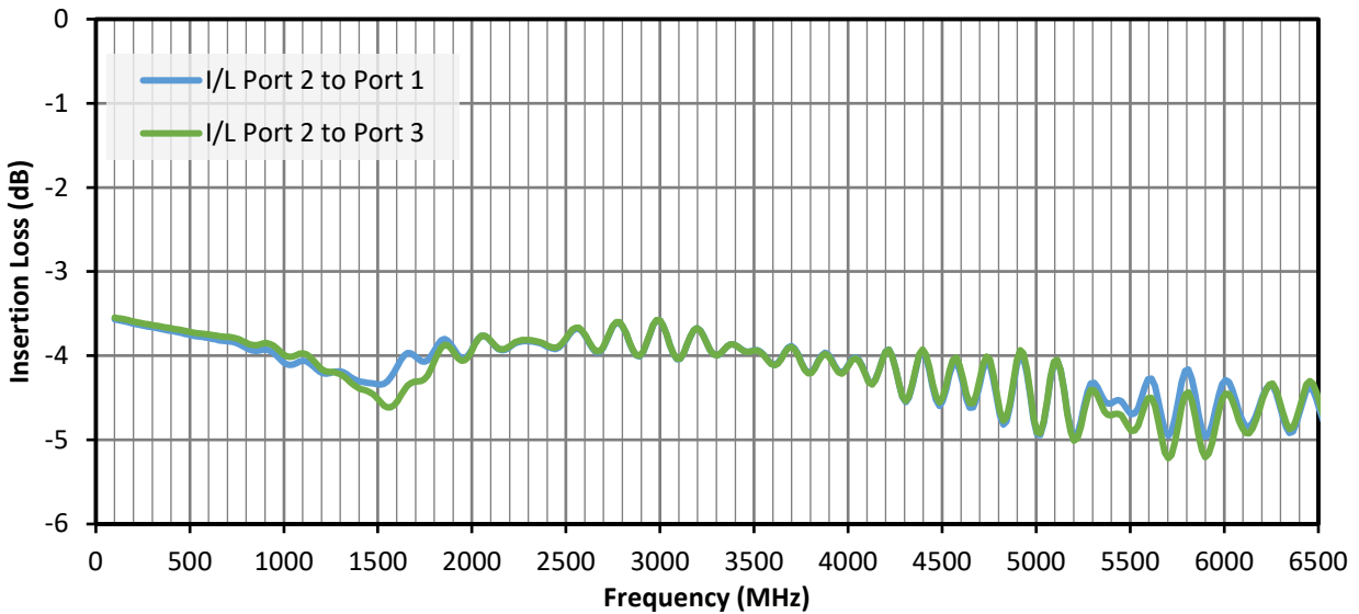
Figure 2. Insertion Loss for the ADP-BNCM-BNCF-T Adapter
