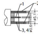
MATING PLUG Jack Insertion Depth 9.1 mm
