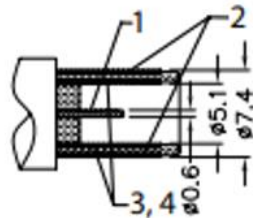
MATING PLUG Jack Insertion Depth 9 mm
