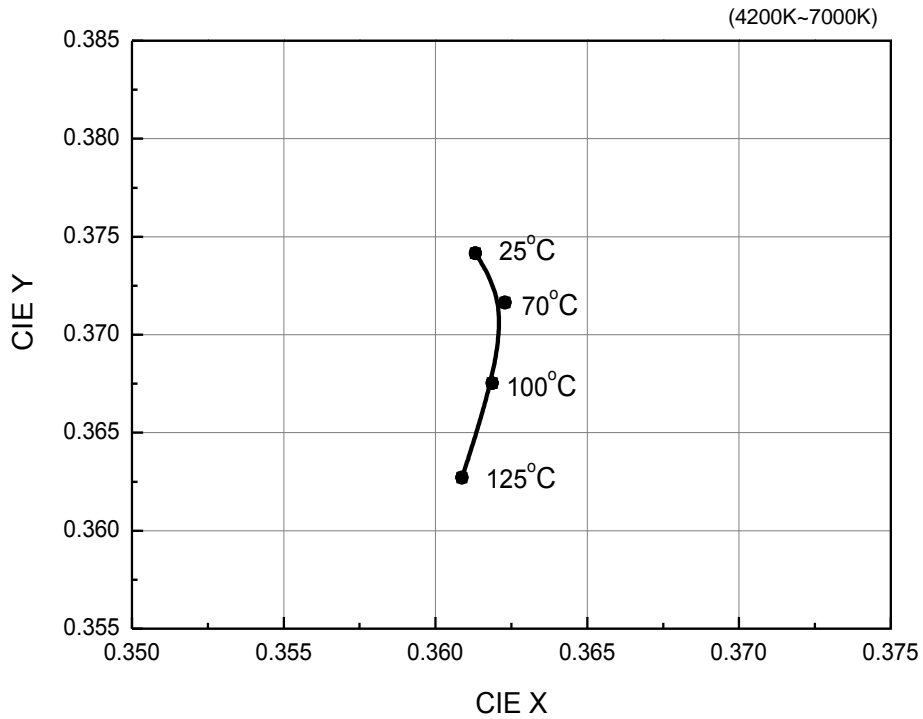
Fig 8. Chromaticity Coordinate vs. Junction Temperature, I_F=150mA
