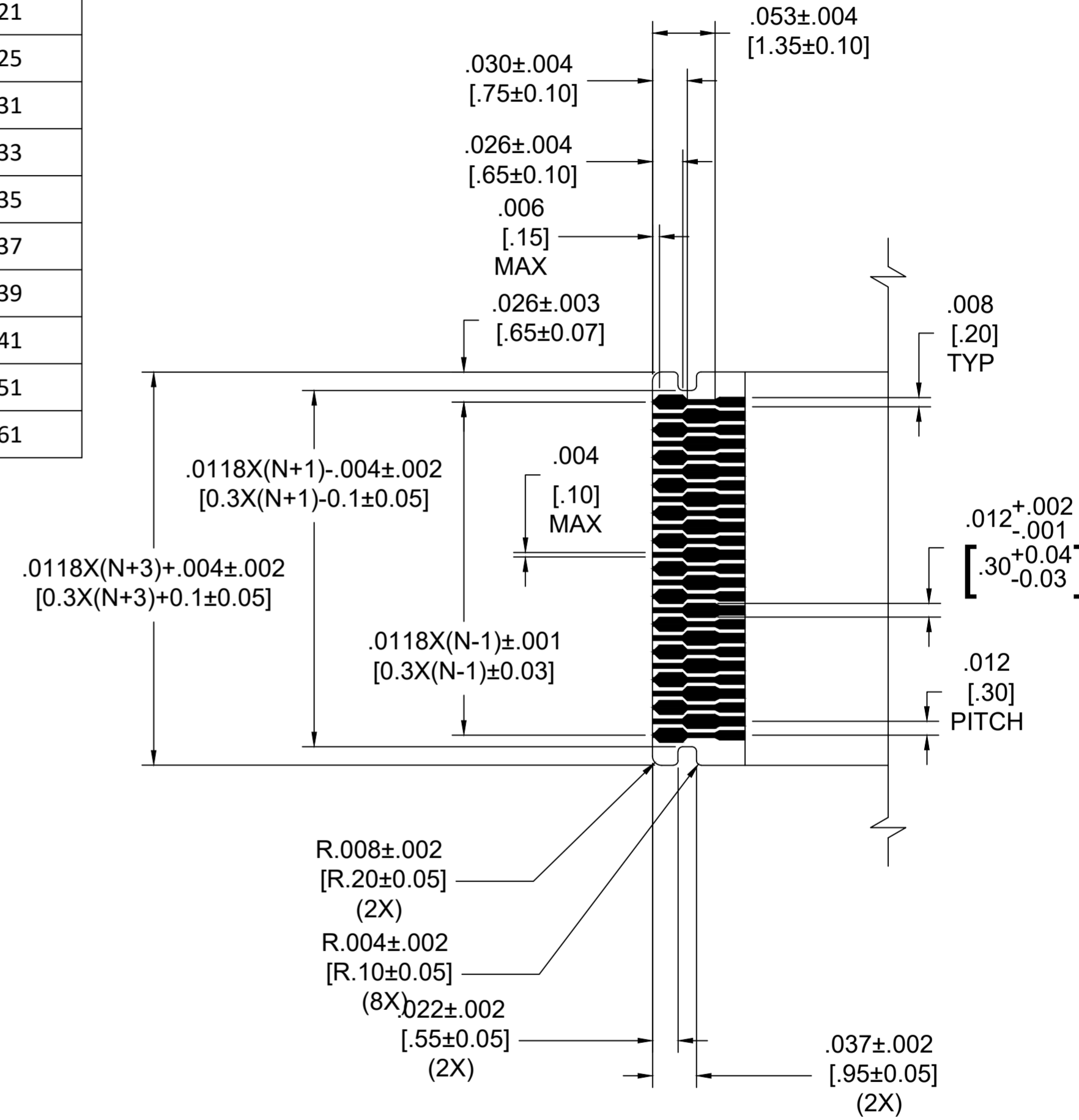
JUMPER END DETAIL 25 CIRCUIT SHOWN (SCALE 10:1)
