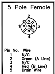
Face View (Typ.)
