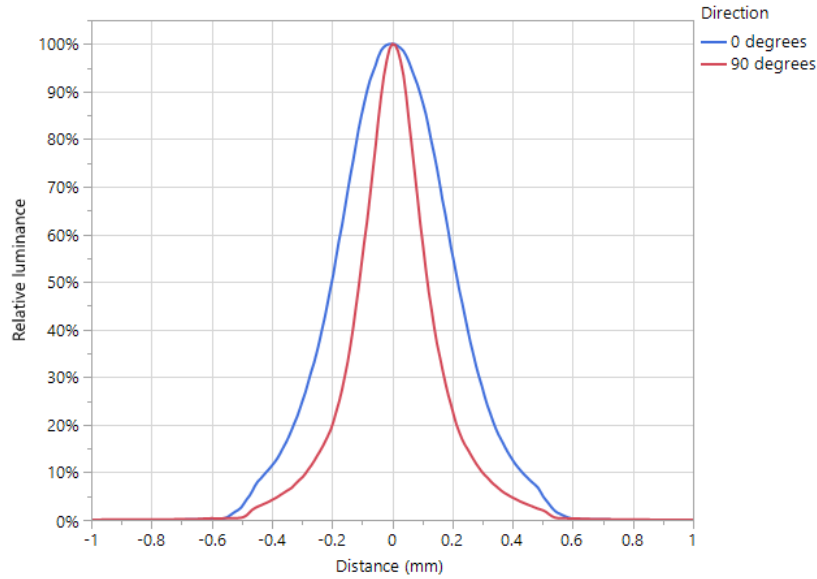
Figure 11: Near field relative luminance (Measured at I_f = 1.65A and at T_{case} = 50^{\circ}C , normalized to 0,0 position)
