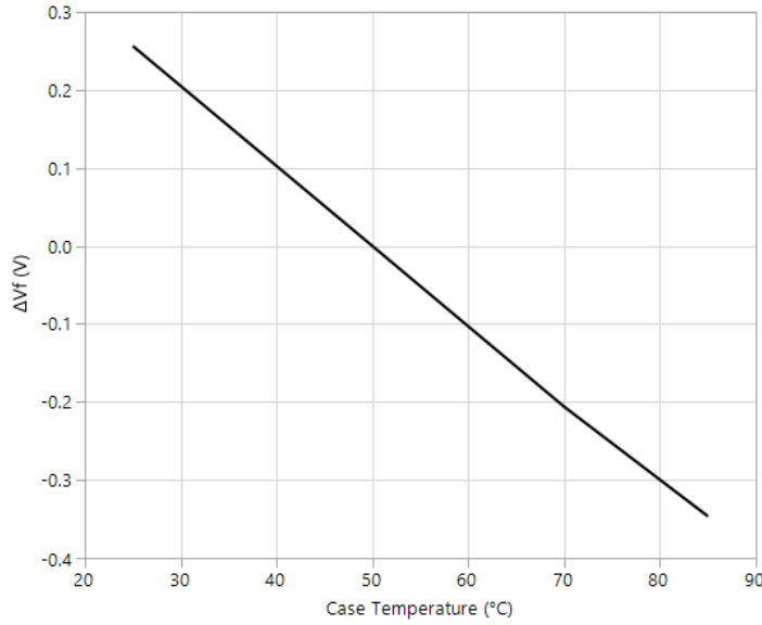
Figure 06: Normalized forward voltage vs temperature (Measured at I_f = 1.65A and normalized at T_{case} = 50^\circ C )
