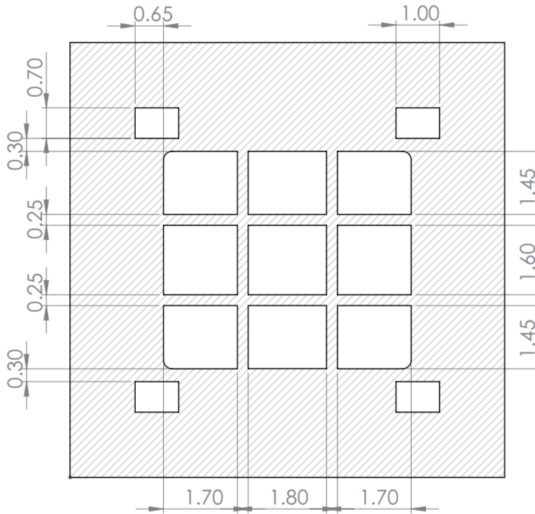
Figure 08: Recommended stencil mask design
