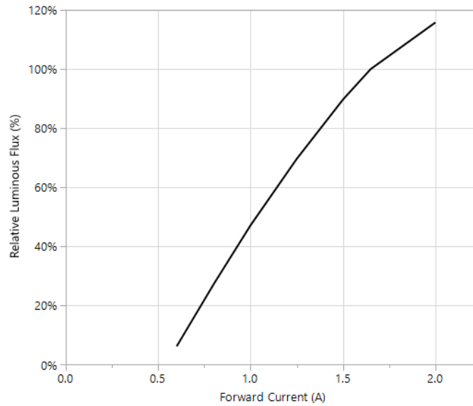
Figure 03: Relative flux vs Current (Normalized luminous flux at I_f = 1.65A and at T_{case} = 50^\circ C )
