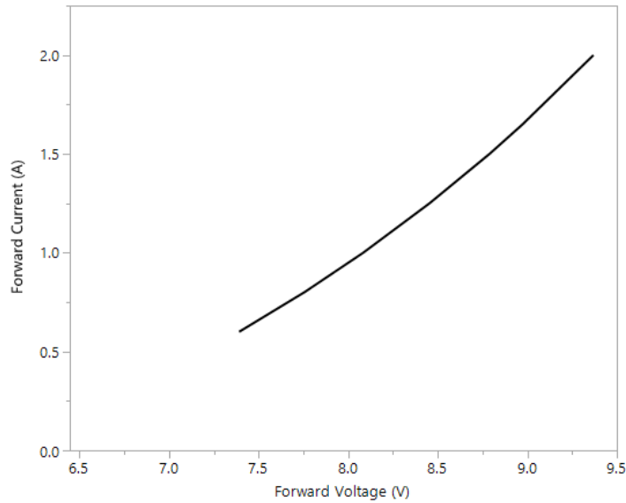
Figure 07: Forward current vs forward voltage (Measured at T_{case} = 50^\circ C )
