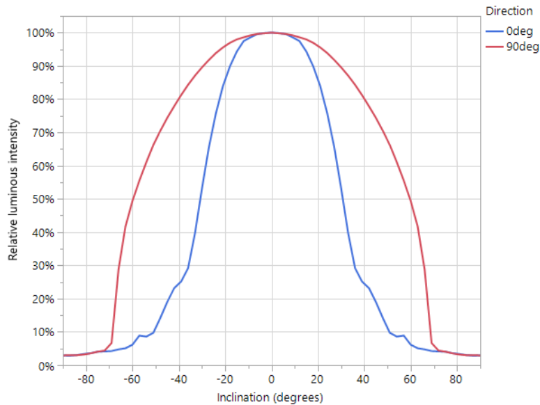
Figure 10: Far field distribution (Measured at I_f = 1.65A and at T_{case} = 50^\circ C , normalized to 0,0 position)
