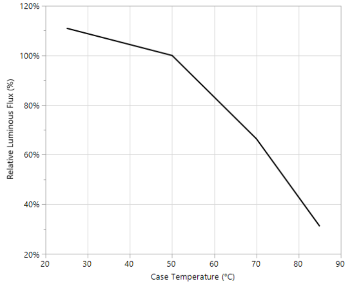
Figure 04: Relative flux vs temperature (Normalized luminous flux at I_f = 1.65A and at T_{case} = 50^{\circ}C )
