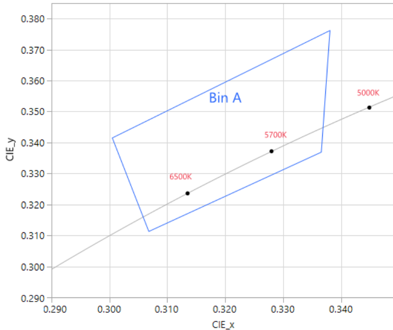
Figure 01: Chromaticity bin plotted with Black Body curve
