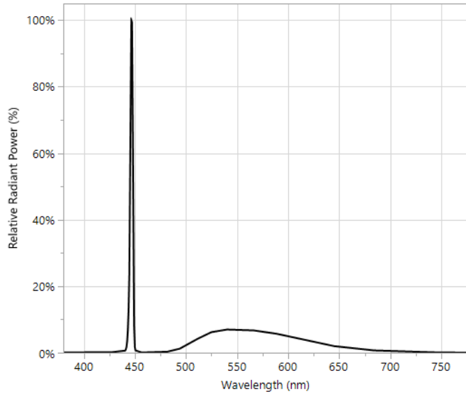
Figure 02: Typical spectral power distribution of 6500K component ( I_f = 1.65A , T_{case} = 50^\circ C )
