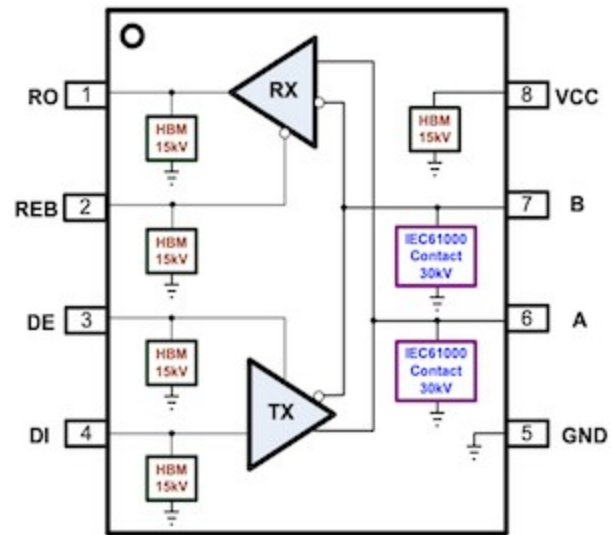
Functional Block of AZRS6534
